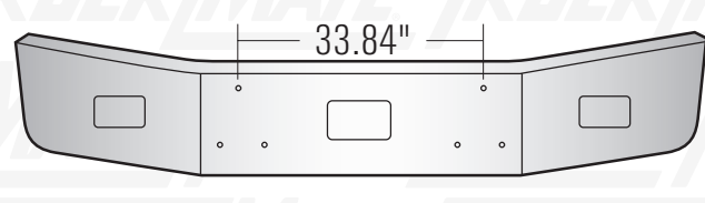
Conv. Model 377SBFA Forward Axle Check Measurements. 1997 & Newer
