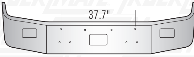
Conv. Model 377SBFA - Check Measurements 1996 & Older
